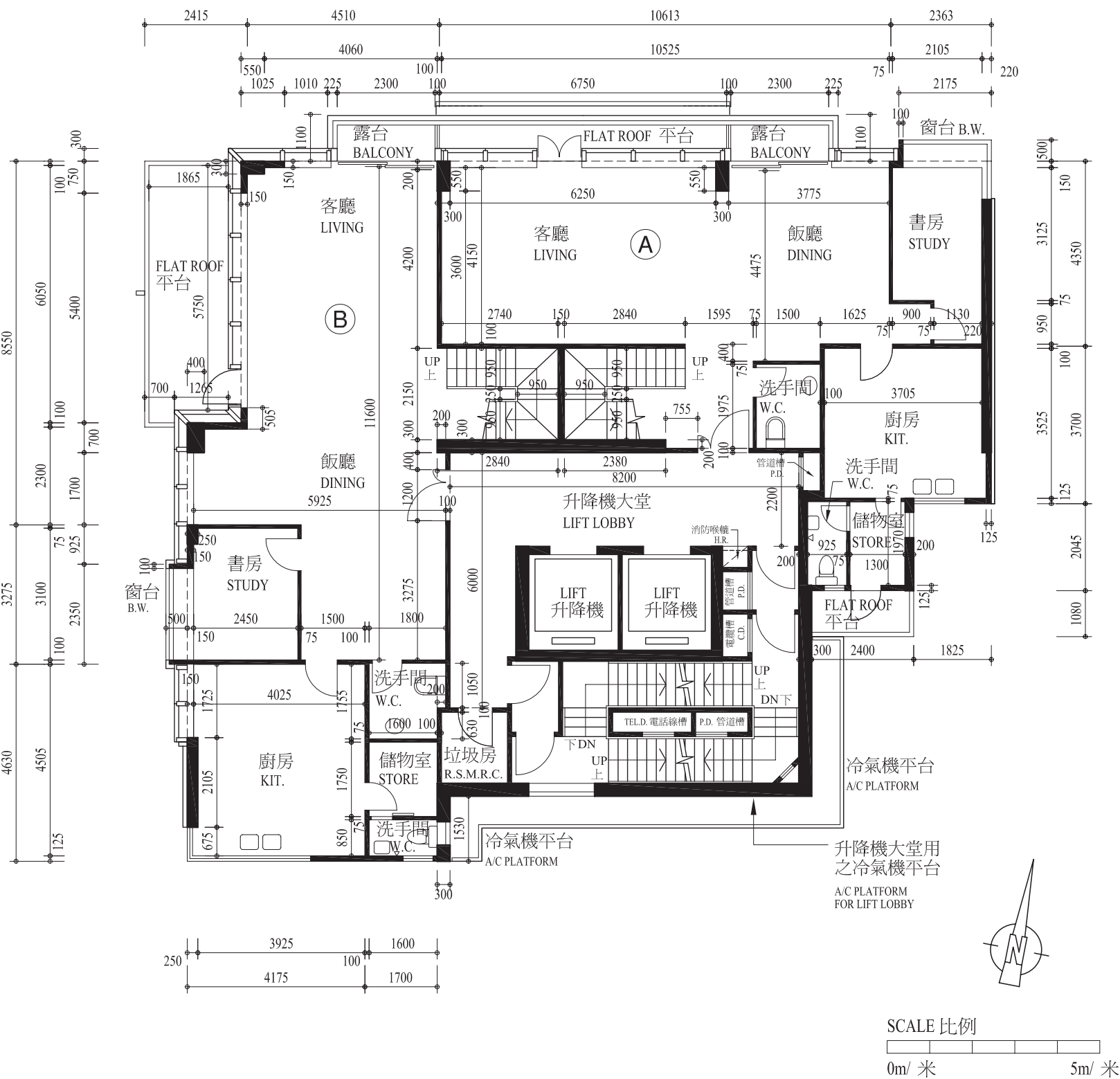
26/F Floor Plan (Lower Duplex) 26樓平面圖(複式低層)
